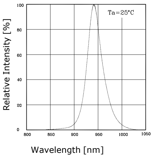
Fig.3 Spectrum Distribution
