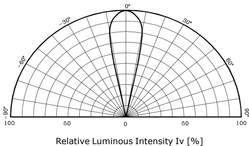
Fig.5 Radiation Characteristics
