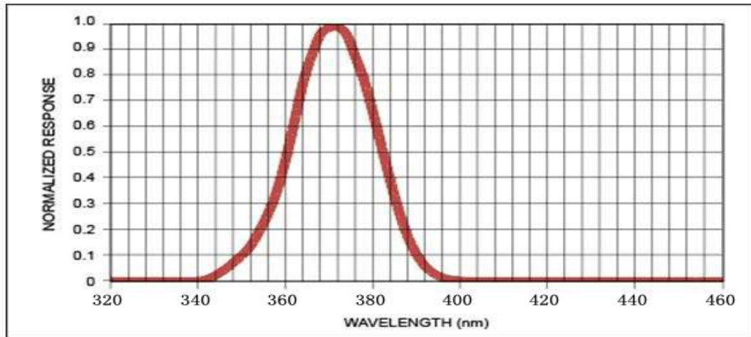
(Optical-Electrical Characteristic)
