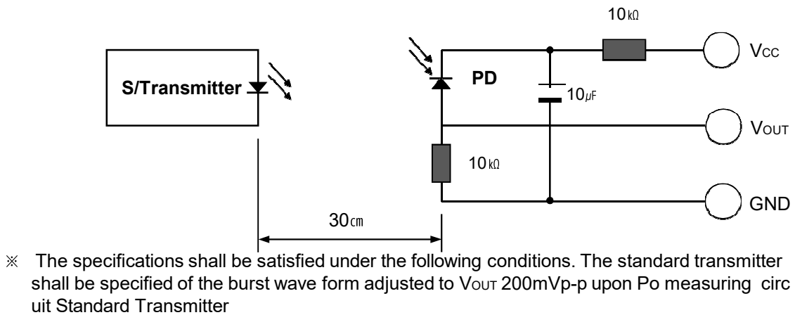
[ Fig.2 ] Transmitter
