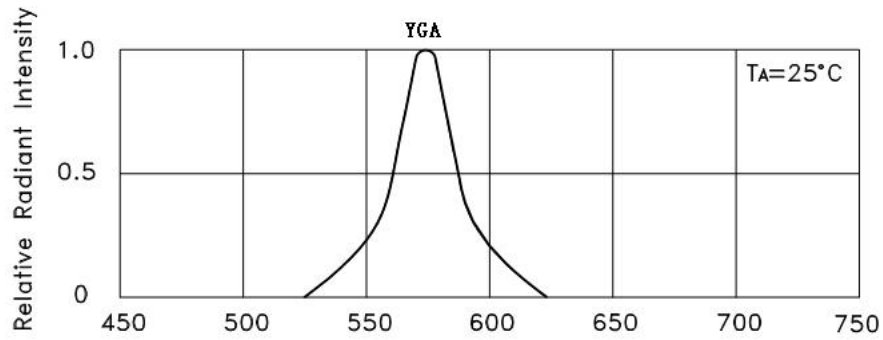
wavelength \lambda (nm) RELATIVE INTENSITY Vs. WAVELENGTH
