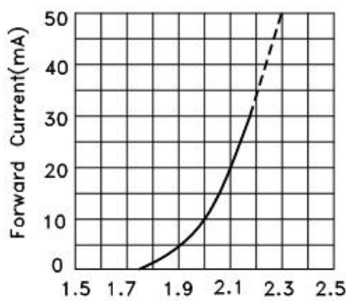
Forward Voltage(V) FORWARD CURRENT Vs. FORWARD VOLTAGE
