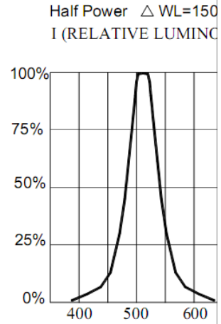
FIG.4 RELATIVE LUMINOUS INTENSITY VS. WAVELENGTH.
