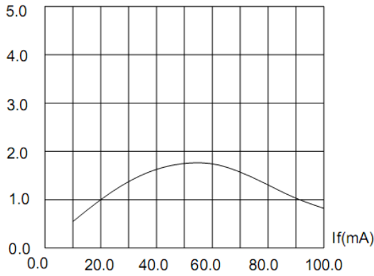
FIG.3 RELATIVE LUMINOUS INTENSITY VS. FORWARD CURRENT
