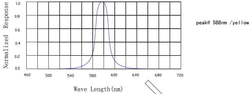
Spectral Reduance
